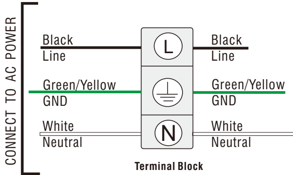
Wire Diagram
