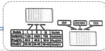
CCT & Power Selectable Slide Switch
