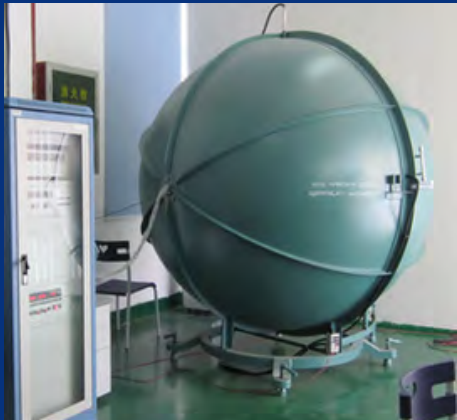
INTEGRATING SPHERE
